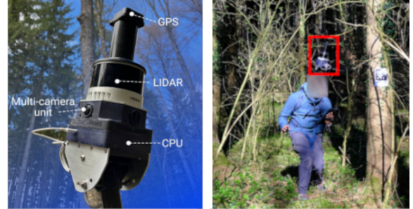
Fig. 3: For the DigiForests dataset, we recorded data with a (left) backpack-carried sensor payload in (right) challenging forest environments with the sensor payload highlighted in red (right).
