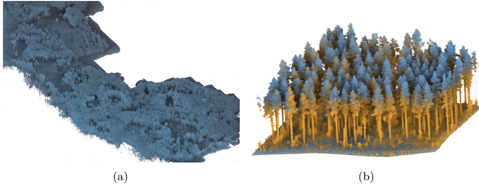
Figure 7: Combination of the (a) aerial point cloud recording of the Stein am Rhein forest region into (b) a complete above-canopy (blue) and below-canopy (yellow) point cloud using the backpack LiDAR data (yellow).
