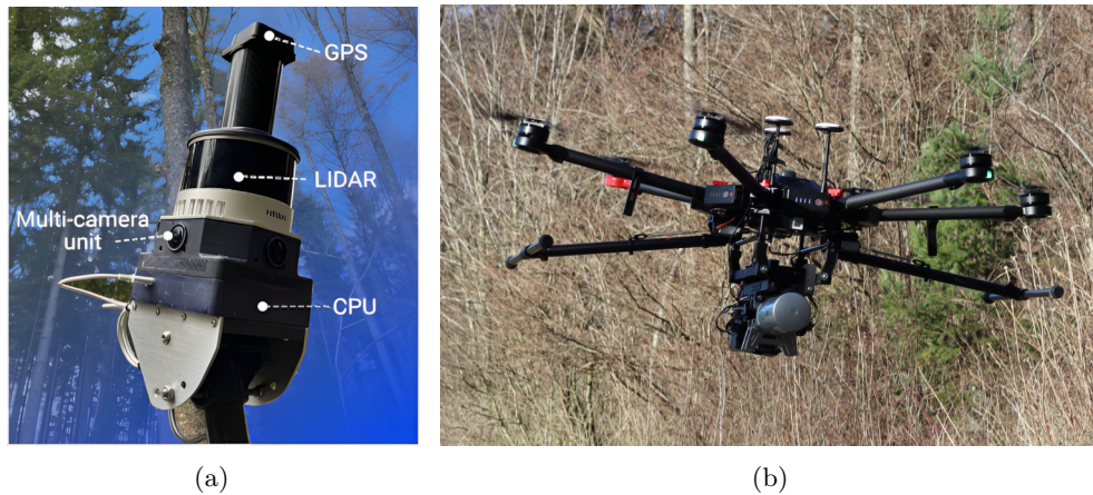
Figure 3: (a) The employed backpack sensor package consisting of the Hesai XT32, the cameras, and the GNSS receiver for geo-referencing the collected data. (b) Aerial drone equipped with a Velodyne HDL-32E in motion recording data.
